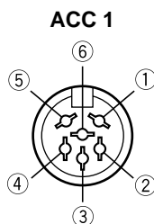
Rear panel view on TS-450S/690S/850S/950SDX
