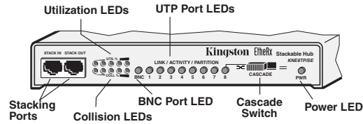
Fig. 1-1 KNE8TP/SE Front Panel
