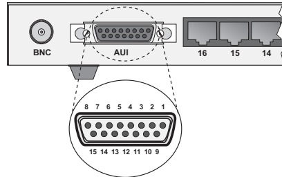
Fig. A-3 AUI Connector on Rear Panel
