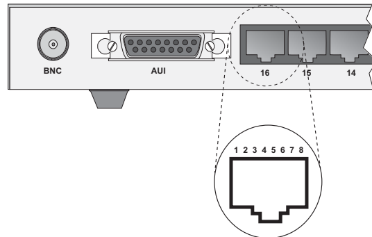
Fig. A-1 RJ-45 Connector Pin Numbers
