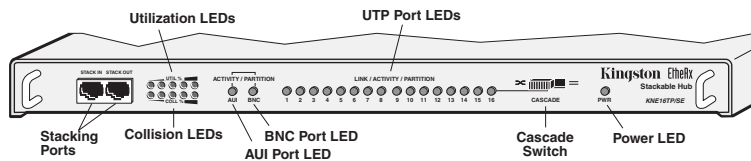
Fig. 1-2 KNE16TP/SE Front Panel
