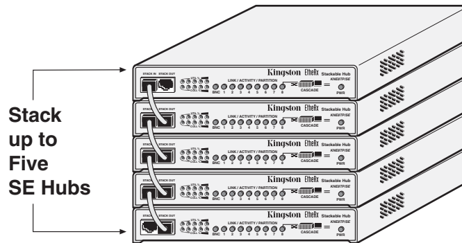
Fig. 3-4 Stackable SE Hub Configuration
