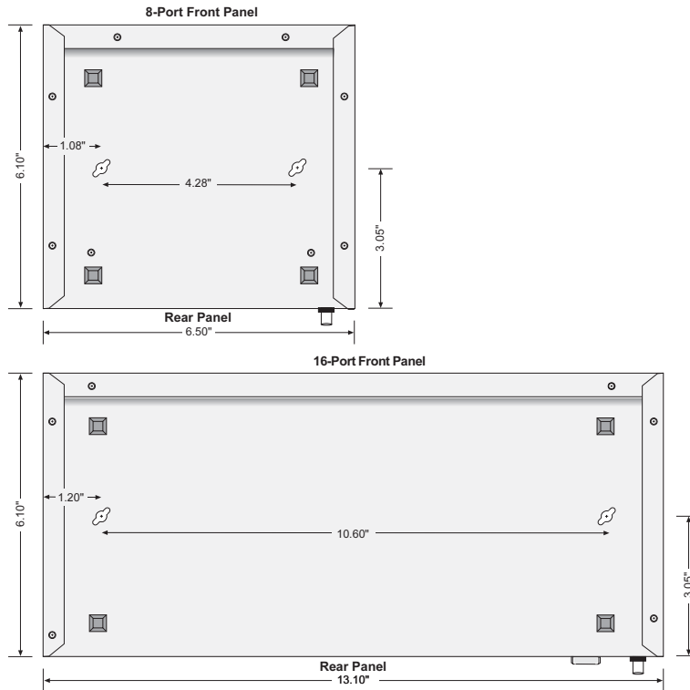
Fig. D-1 Mounting Template specifications
