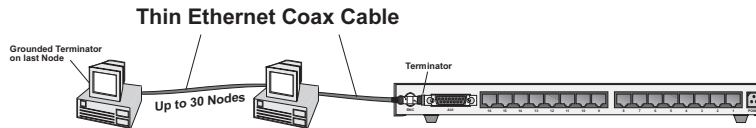
Fig. 3-2 Linear Bus Connection
