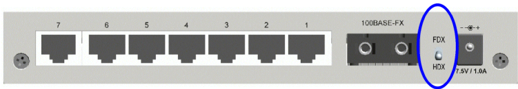
100FX Duplex Selector
