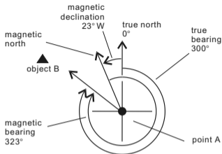
Compensate the Bearing at a place with Westerly (W) Magnetic Declination
