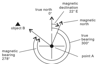
Compensate the Bearing at a place with Easterly (E) Magnetic Declination
