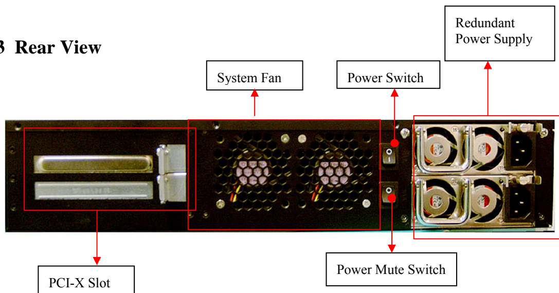
Figure 6 – FW-7890 Rear View
