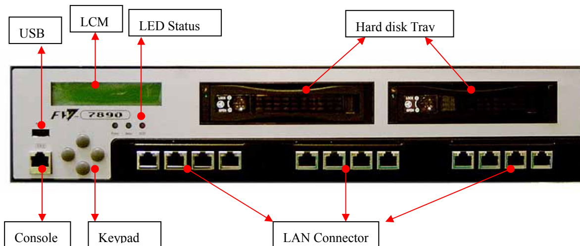
Figure 5 – FW-7890 Face Panel
