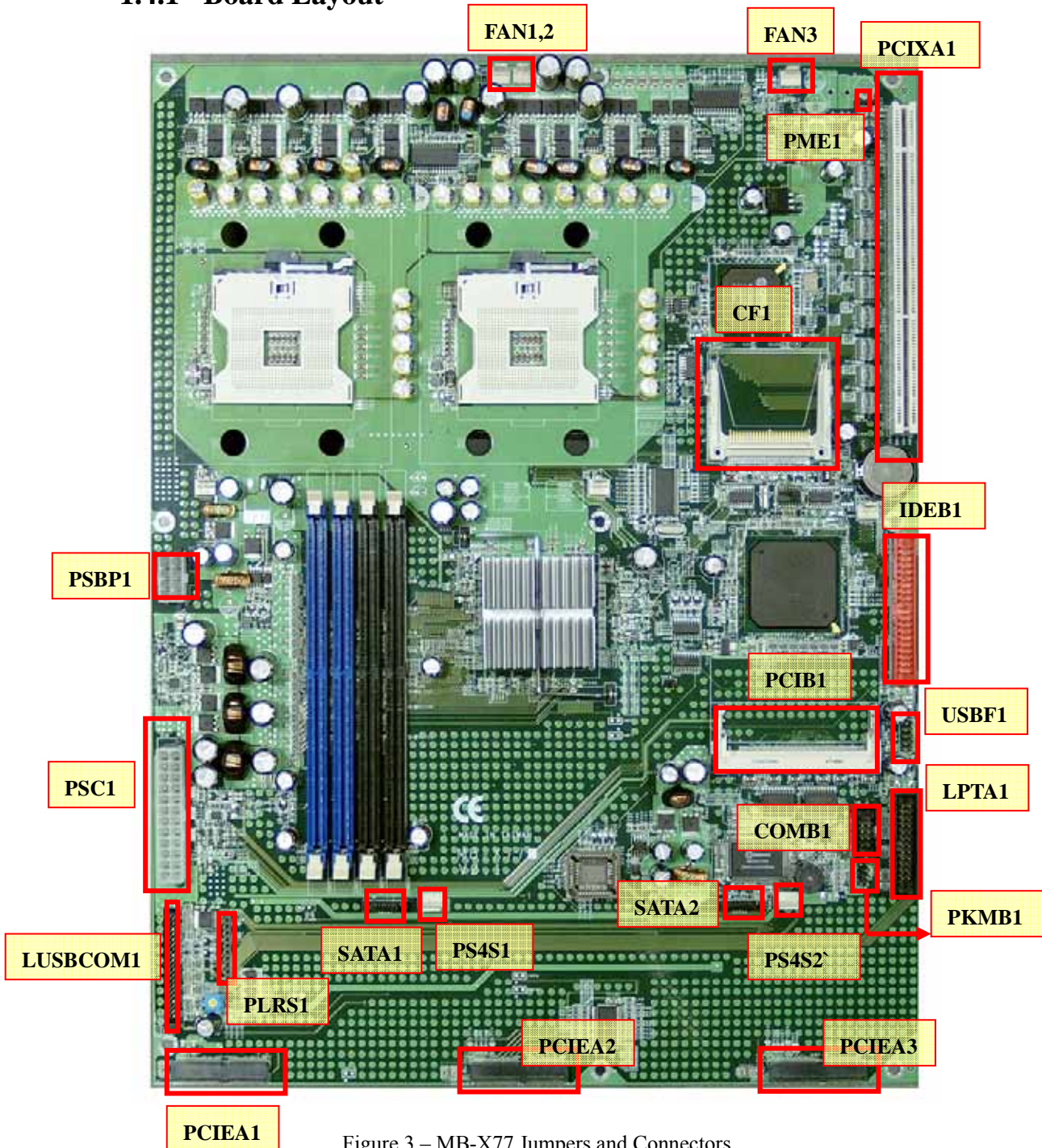
Figure 3 – MB-X77 Jumpers and Connectors
