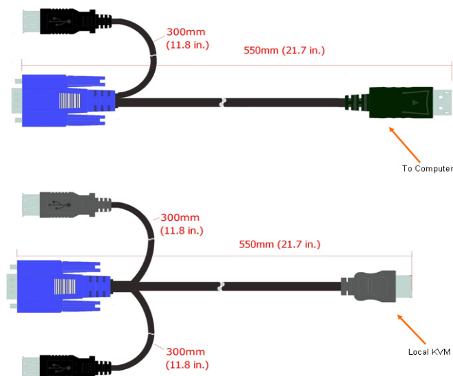
Figure 2-6 SpiderDuo USB Cable Dimensions
