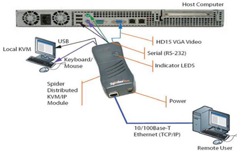
Figure 2-4 SpiderDuo System Configuration
