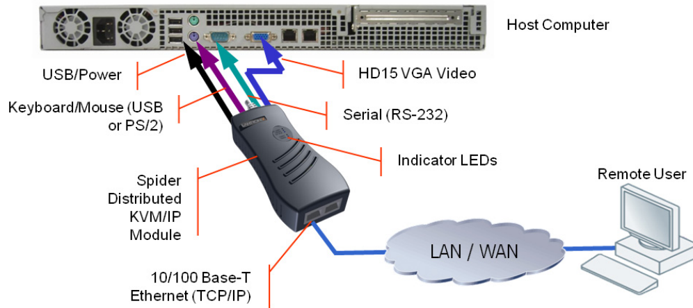
Figure 2-1 Spider System Configuration
