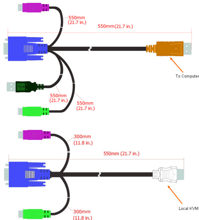
Figure 2-5 SpiderDuo PS/2 Cable Dimensions
