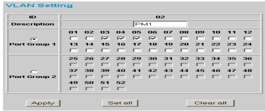
Figure 20. VLAN Settings
