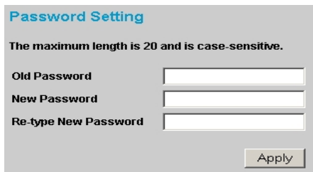
Figure 10. Password Change
