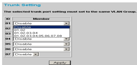
Figure 22. Trunk Settings
