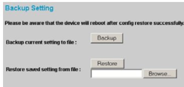
Figure 28. Backup Setting
