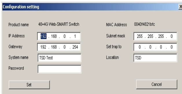
Figure 9. Configuration Setting
