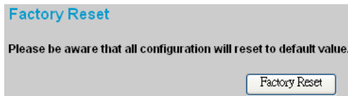
Figure 29. Reset Setting
