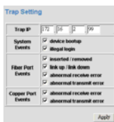
Figure 26. Trap Setting
