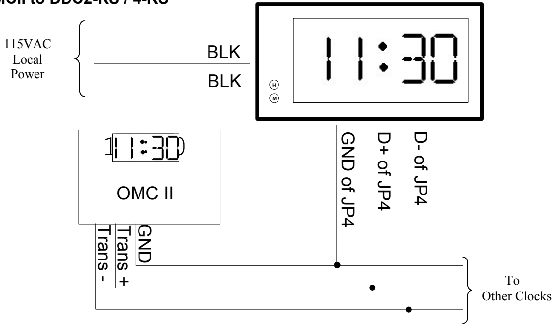
OMCII DB9 Female Plug
