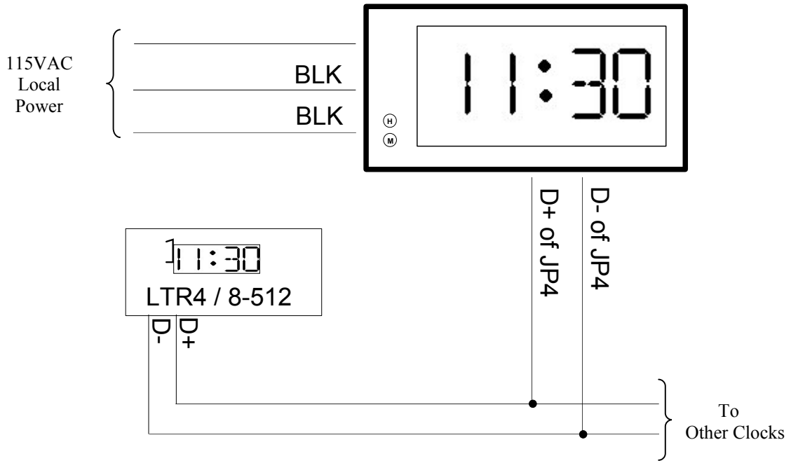
LTR4 / 8-512 Terminal Connections
