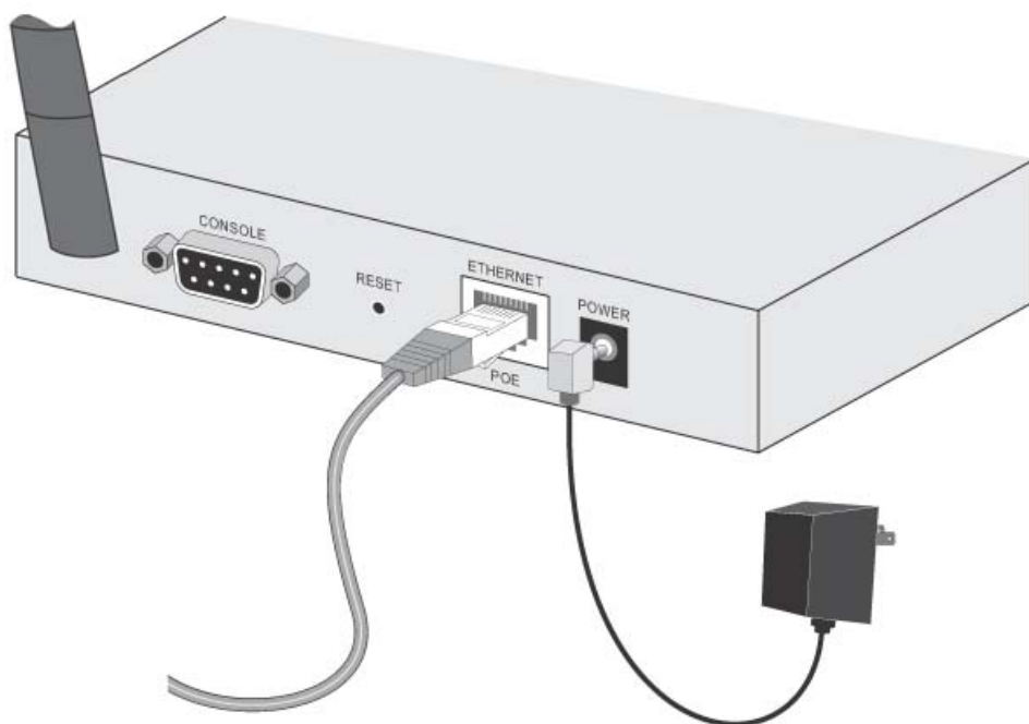
Figure 4: Installation Diagram
