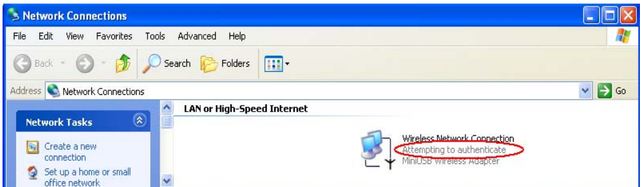
Figure 5: Authenticating
