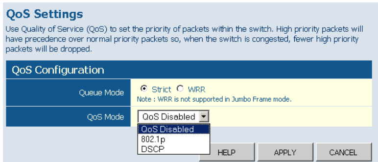
Figure 5-24 QoS Settings
