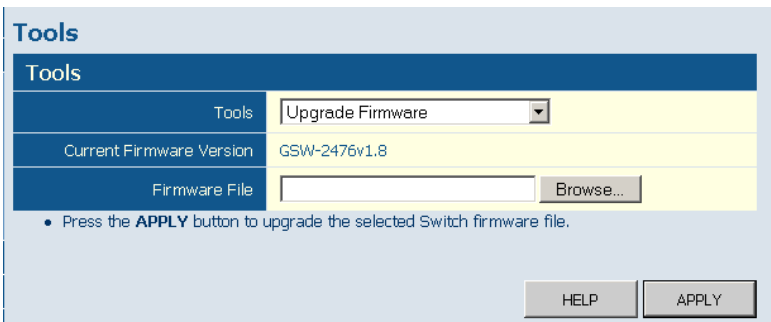
Figure 5-9 Upgrade Firmware
