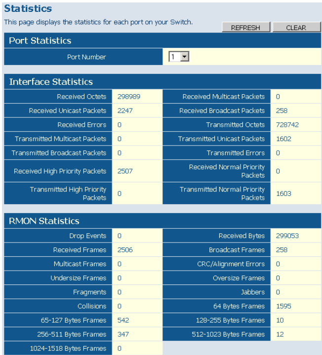
Figure 5-4 Port Statistics
