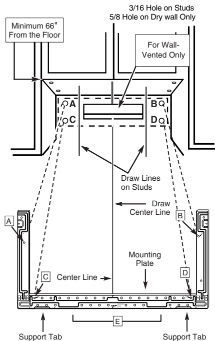
(3 pieces mounting plate)
