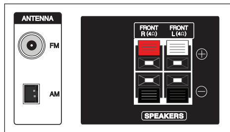
BACK PANEL
