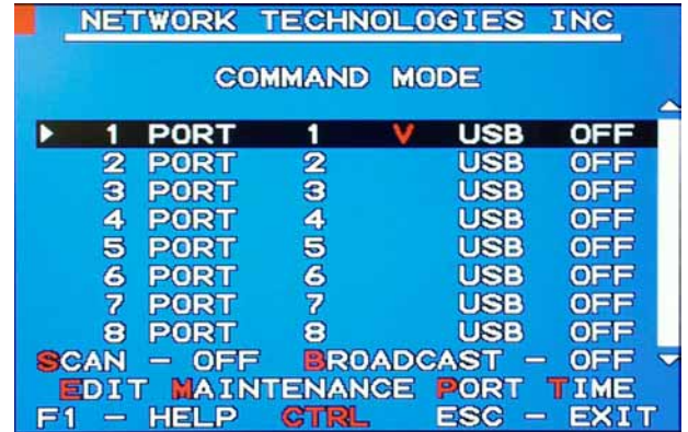
Figure 15- More Command Mode Features
