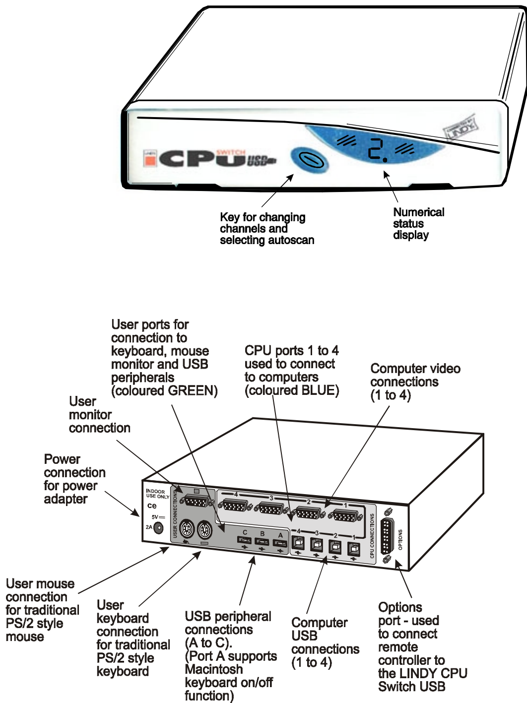
Fig. 1 – LINDY CPU Switch USB model 32 341
