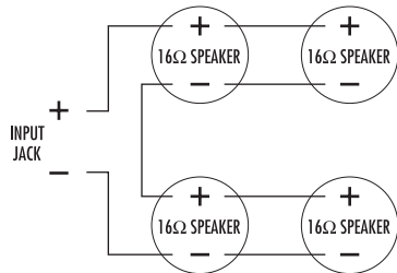
Typical 16 Ohm Wiring Setup
