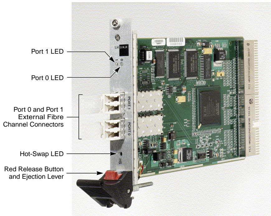
Figure 2.1 LSI7202CP CompactPCI Host Adapter
