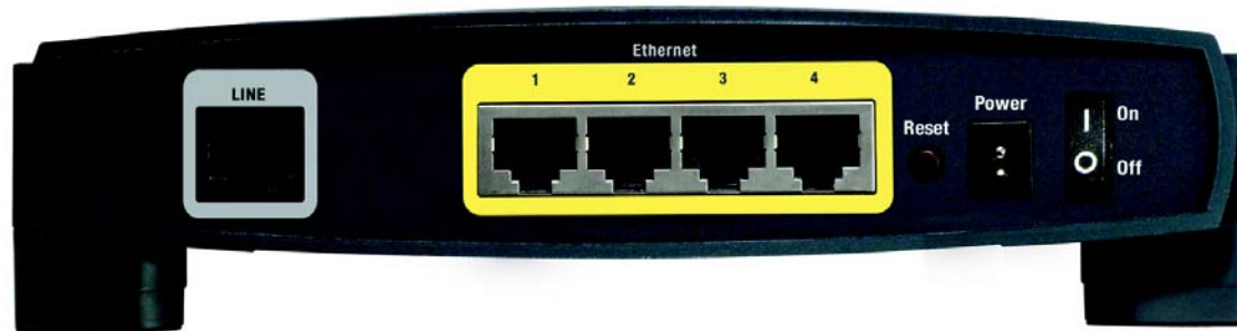
Figure 3-1: Back Panel
