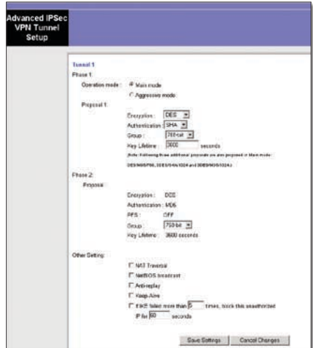
Advanced VPN Tunnel Setup
