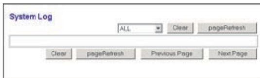
System Log
