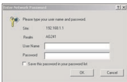
Login Screen
