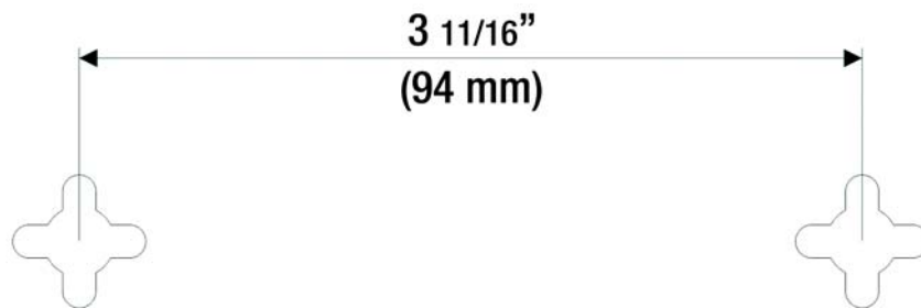
Figure C-4: Wall-Mounting Hardware
