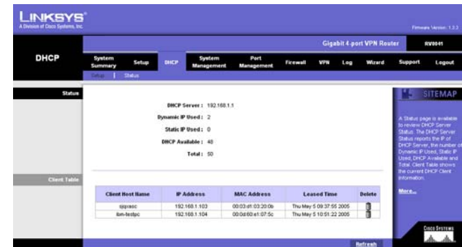
Figure 5-22: DHCP Status
