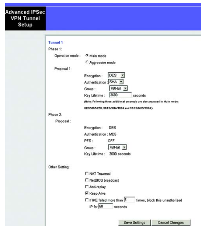
Figure 4-29: Advanced VPN Tunnel Setup
