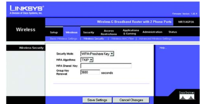
Figure 5-11: Wireless Tab - Wireless Security (WPA Pre-Shared Key)
