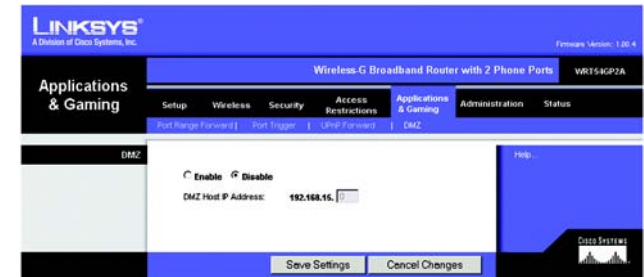
Figure 5-27: Applications & Gaming Tab - DMZ
