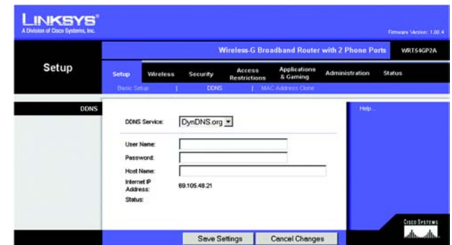
Figure 5-7: Setup Tab - DDNS (DynDNS.org)
