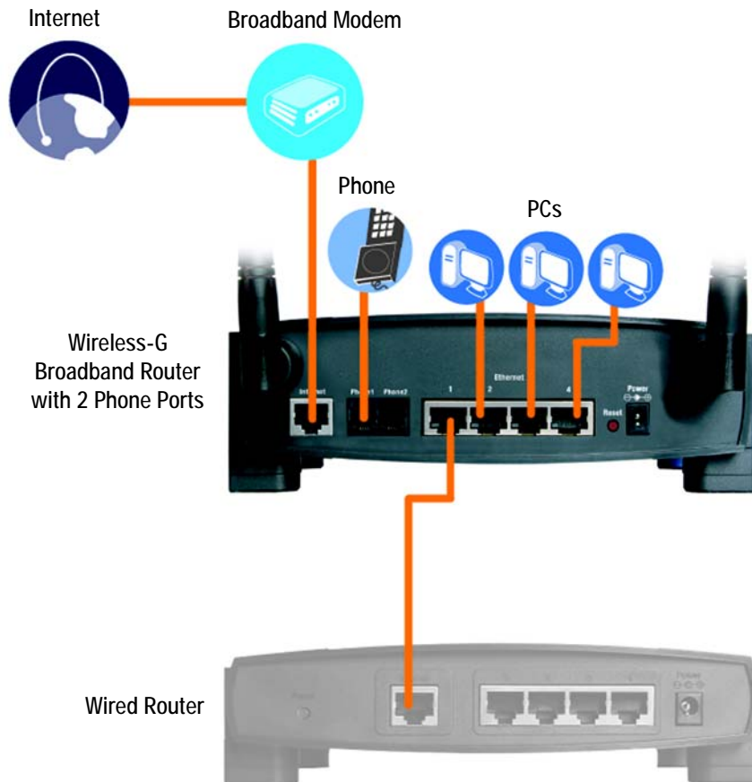
Figure 4-5: Router Connected to Another Router
