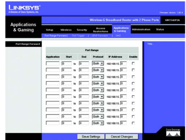
Figure 5-24: Applications & Gaming Tab - Port Range Forward
