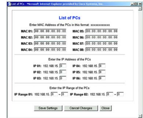
Figure 5-23: List of PCs
