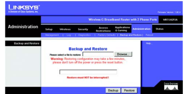
Figure 5-34: Administration Tab - Backup and Restore
