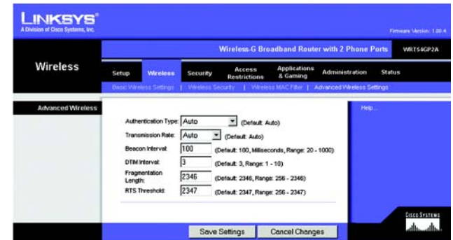
Figure 5-18: Wireless Tab - Advanced Wireless Settings
