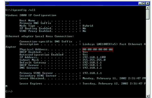
Figure D-3: MAC Address/Physical Address
