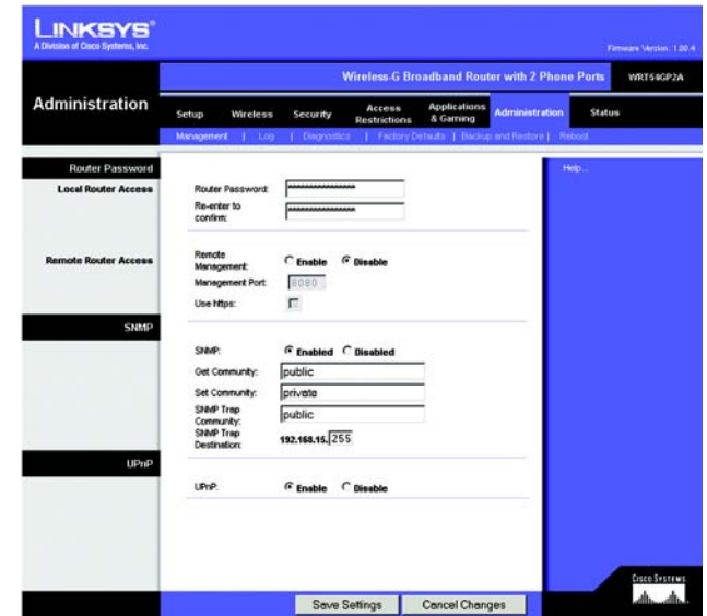
Figure 5-28: Administration Tab - Management
