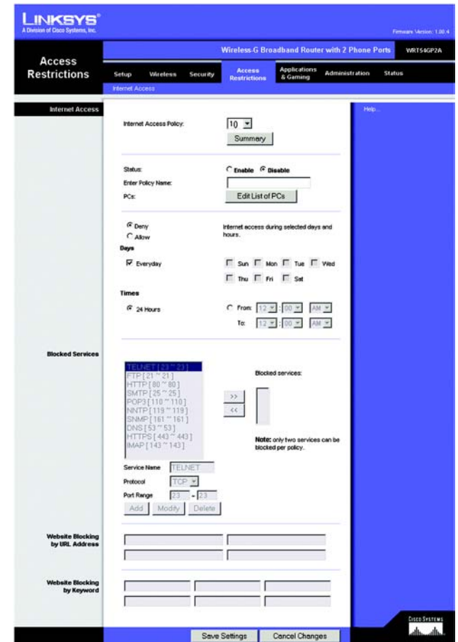
Figure 5-21: Access Restrictions Tab - Internet Access
