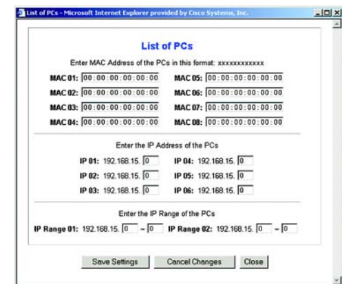
Figure D-4: Access Restrictions - MAC and IP Addresses
