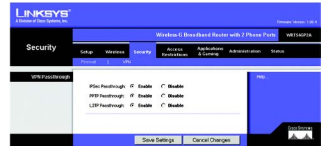
Figure 5-20: Security Tab - VPN
