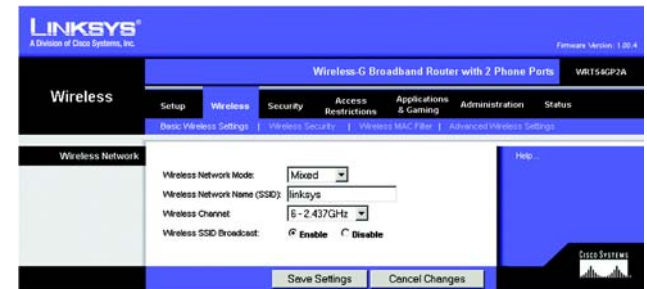
Figure 5-10: Wireless Tab - Basic Wireless Settings
