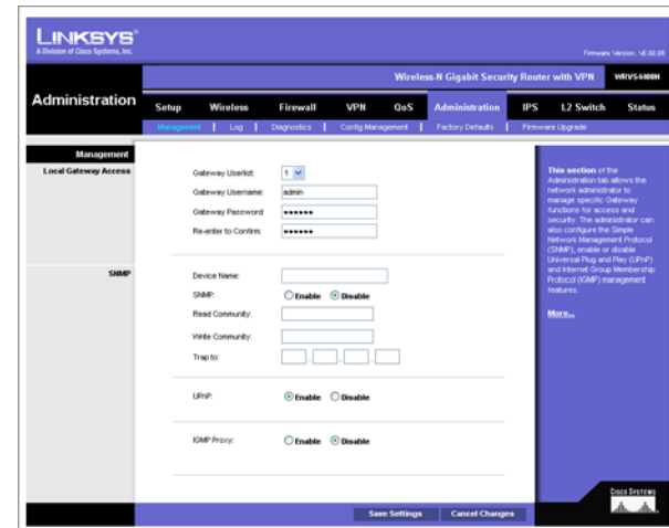
Figure 6-49: Administration - Management
