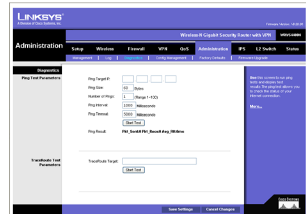
Figure 6-52: Administration - Diagnostics
