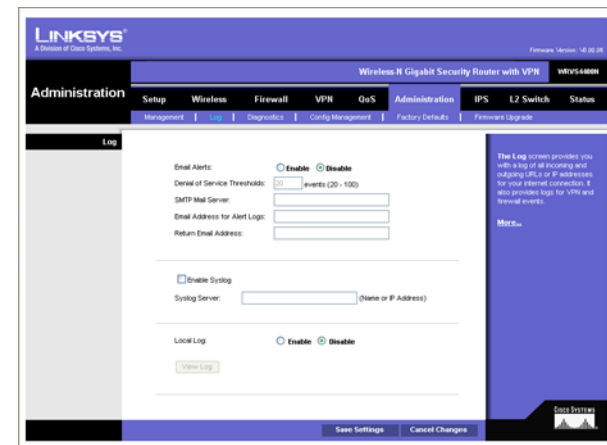
Figure 6-50: Administration - Log
