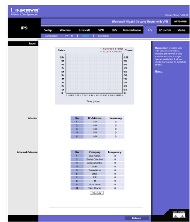
Figure 6-60: IPS - Report
