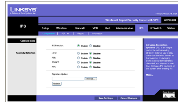
Figure 6-58: IPS - Configuration
