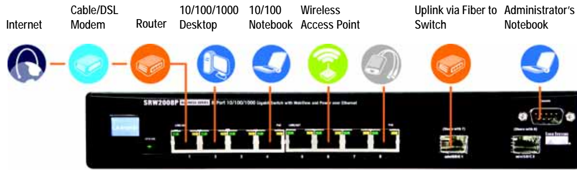
Figure 3-1: Typical Network Configuration for the SRW2008P
