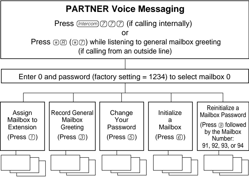
Figure 2. Programming Menu
