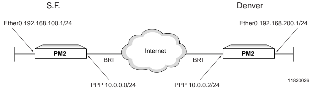
Figure 12-3 ISDN BRI Numbered
