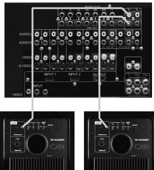
Preamplifier Processor (Unbalanced RCA to Unbalanced RCA)
