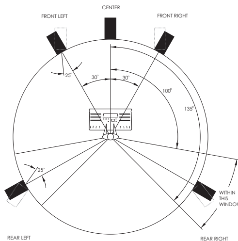
Surround placement
