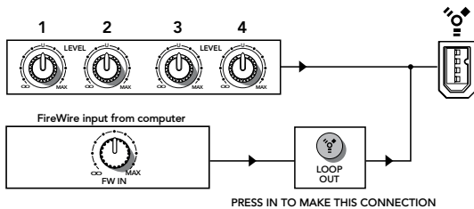
FireWire recording channels 1–4 and FireWire in
