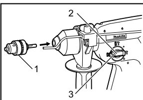
1. Drill chuck 2. Change lever 3. Pointer
