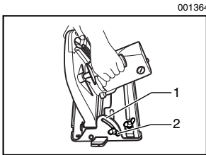
1. Bevel scale plate 2. Clamping screw
