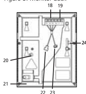
Figure 5. Monitor back
