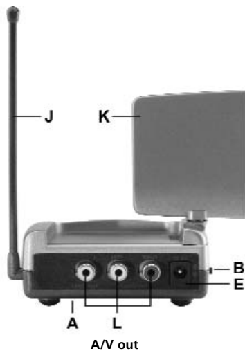
Figura 4 RECEPTOR A/V
