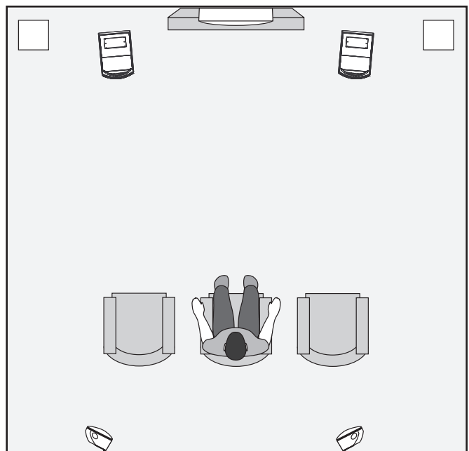
Figure 14. Purity speakers as front channels, Vignette speakers above the television and along the back wall as the center and surround (effects) channels, and Dynamo subwoofers in the front corners as the 0.1 (effects) channel.
