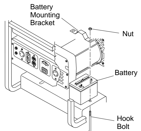
Figure 10 - Battery Hold-Down System (Model MGH7000D Shown)
