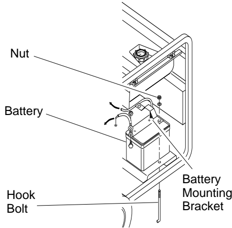
Figure 11 - Battery Hold-Down System (Model MGH10000A Shown)
