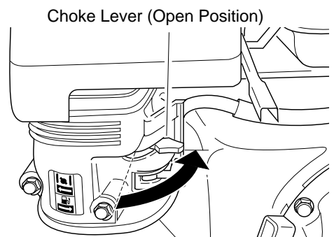
Figure 21 - Choke Lever Opened (Model MGH7000D Shown)
