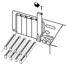
Figure 2-2 Expansion Slots
