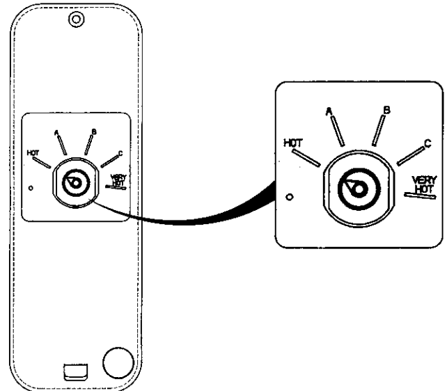
LOWER THERMOSTAT ADJUSTABLE THROUGH OPENING IN LOWER ACCESS PANEL
