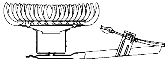
PROPANE (L.P.) GAS BURNER - 40 AND 50 GALLON
