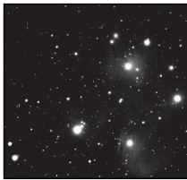
Fig. 35: The Pleiades is one of the most beautiful open clusters.
