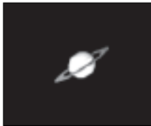
Fig. 33: Saturn has the most extensive ring structure in our Solar System.
