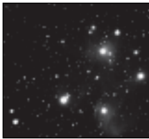
Fig. 34: The Pleiades is one of the most beautiful open clusters.
