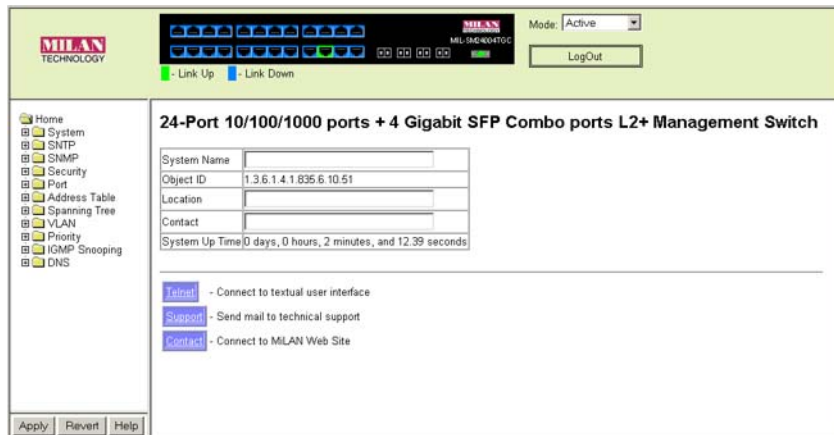
Figure 3-1 Home Page
