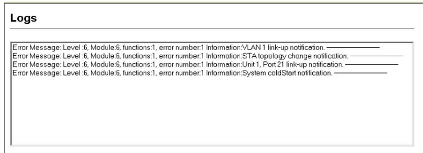
Figure 3-14 Displaying Logs
