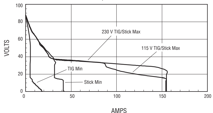
VOLT/AMP CURVES
