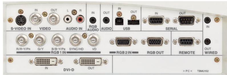
Terminals
