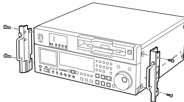
Rack-mounting adaptors
