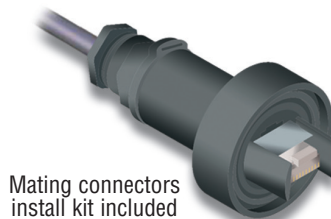
Sealing gland and cage optimized to maintain IP68 seal and provide secure cable restraint without disrupting signal
