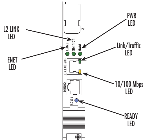
Figure 4. Model 6081RC LEDs
