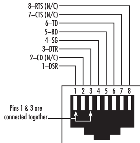
Figure 16. EIA-561 (RJ-45 8-pin) port
