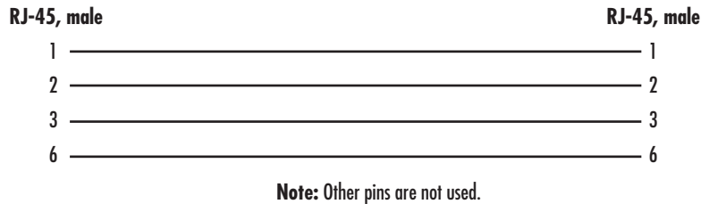
Figure 14. Typical Ethernet straight-through cable diagram for 10/100Base-T
