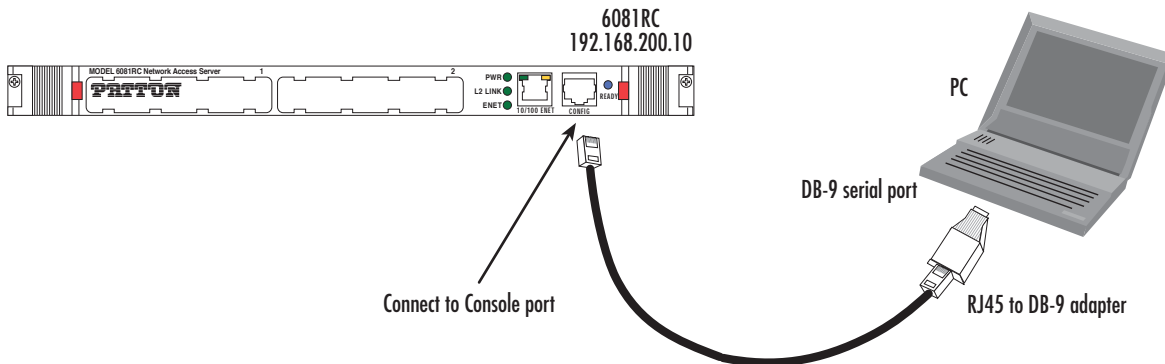
Figure 12. Connecting the 6081RC to your laptop PC via the console port
