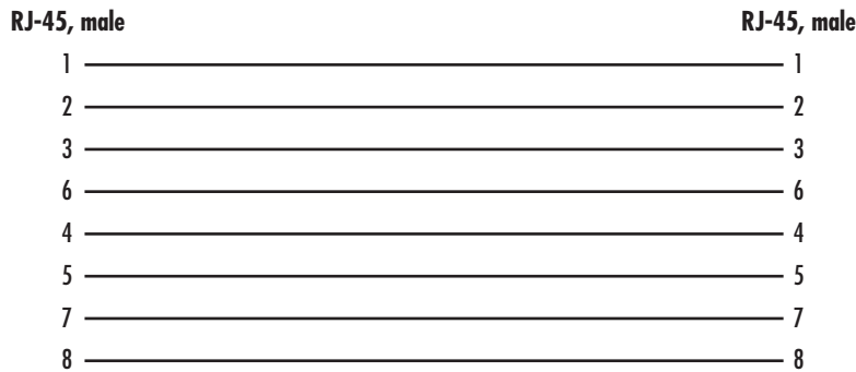
Figure 15. Typical Ethernet straight-through cable diagram for 1000Base-T
