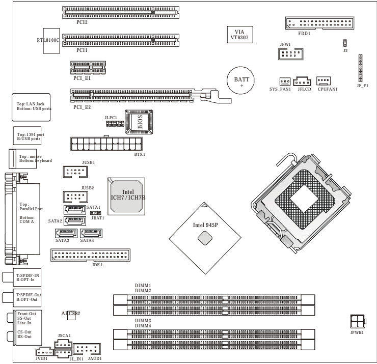
945P Series(MS-7204) v1.x mBTX Mainboard
