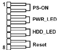
JF_P1 Pin Definition
