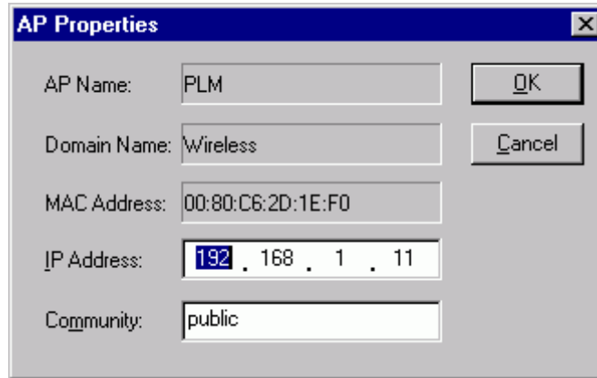
Figure 24. AP Properties
