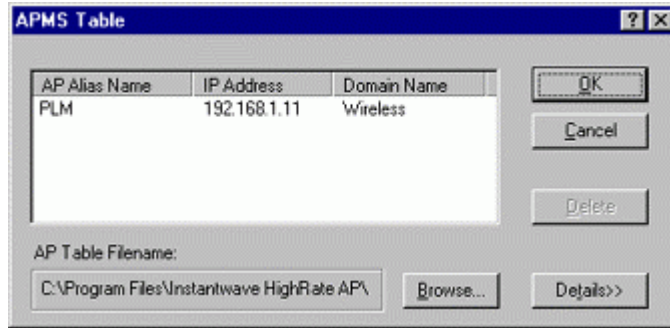
Figure 19. APMS Table-1
