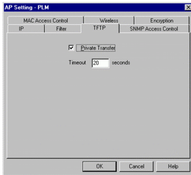
Figure 28. AP Setting/TFTP
