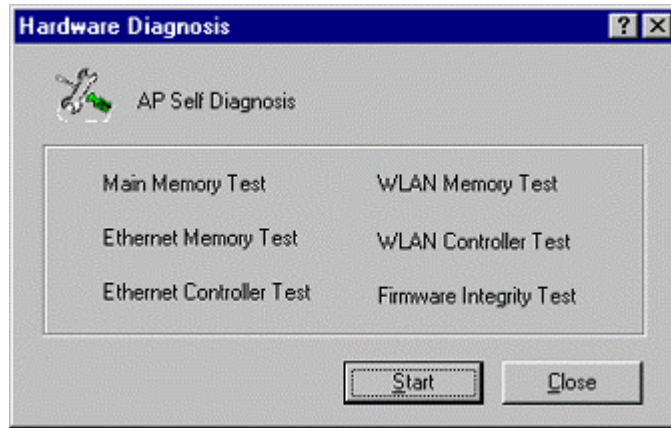
Figure 16. Hardware Diagnosis
