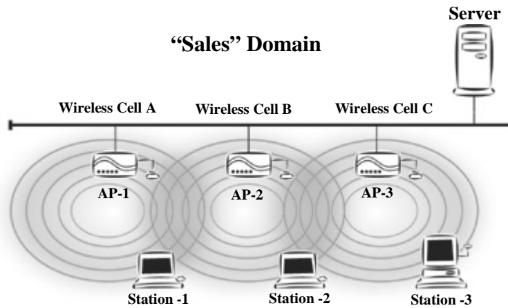
Figure 3. Multiple AP Network
