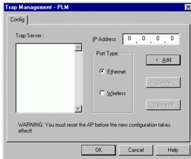
Figure 33. Trap Management
