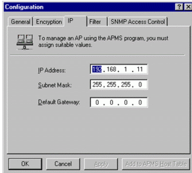
Figure 12. Configuration/IP
