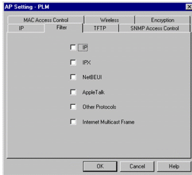
Figure 27. Filter (APMS)
