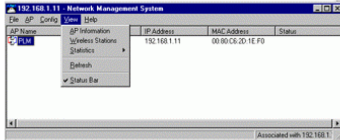
Figure 36. View Menu
