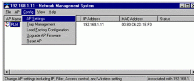
Figure 25. Config/AP Setting
