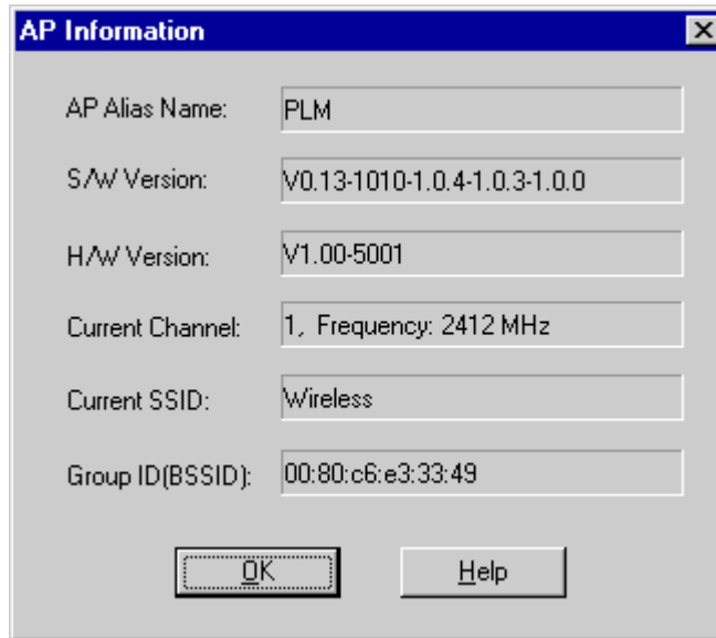
Figure 37. AP Information
