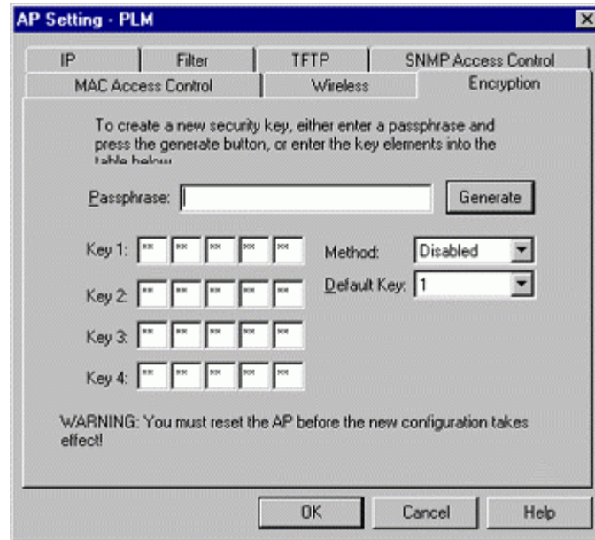
Figure 32. AP Setting/Encryption
