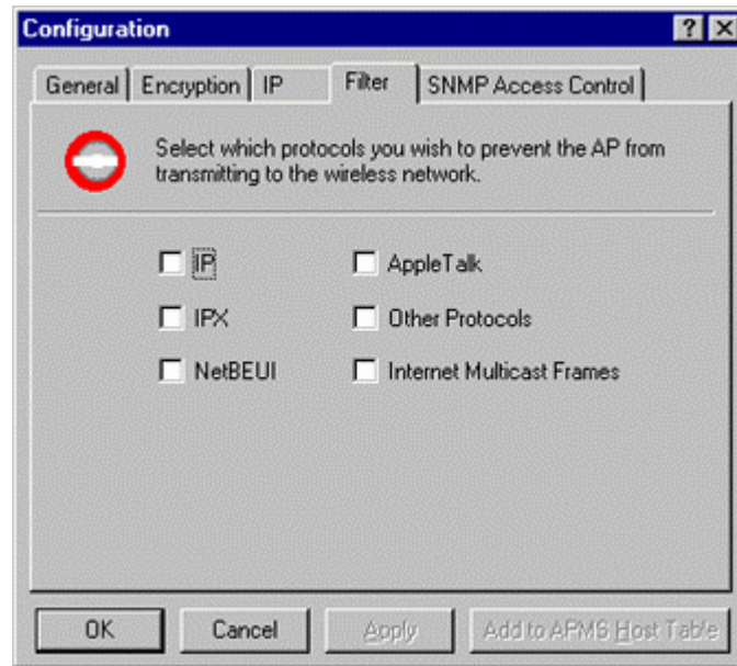
Figure 13. Configuration/Filter
