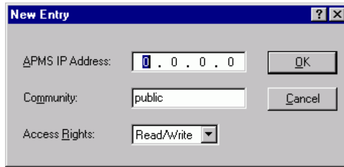
Figure 15. New Entry
