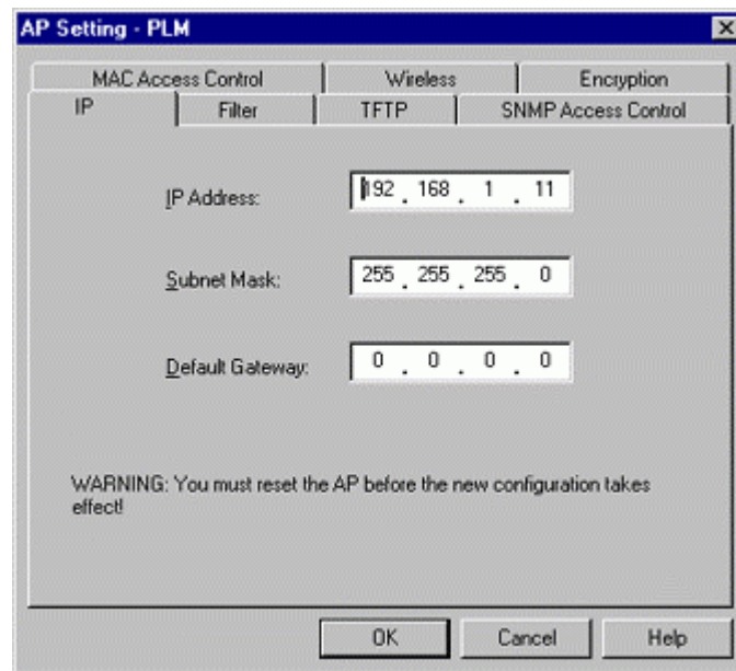
Figure 26. AP Settings/IP
