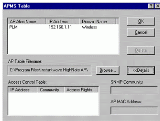
Figure 20. APMS Table-2
