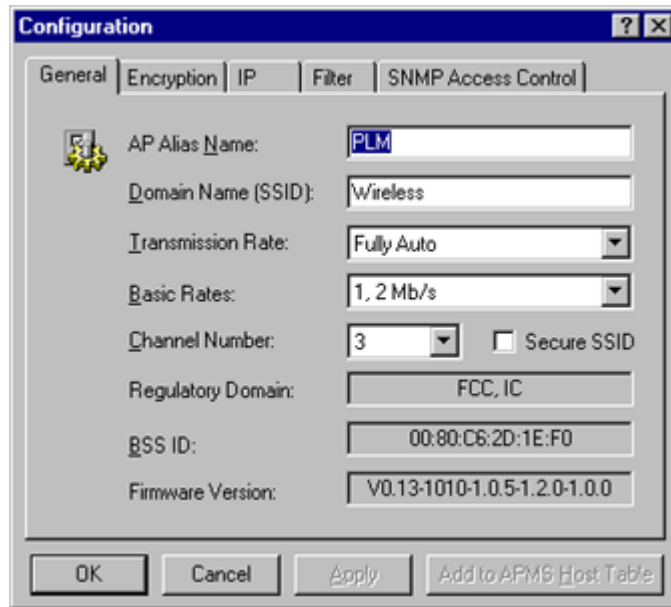
Figure 10. Configuration/General
