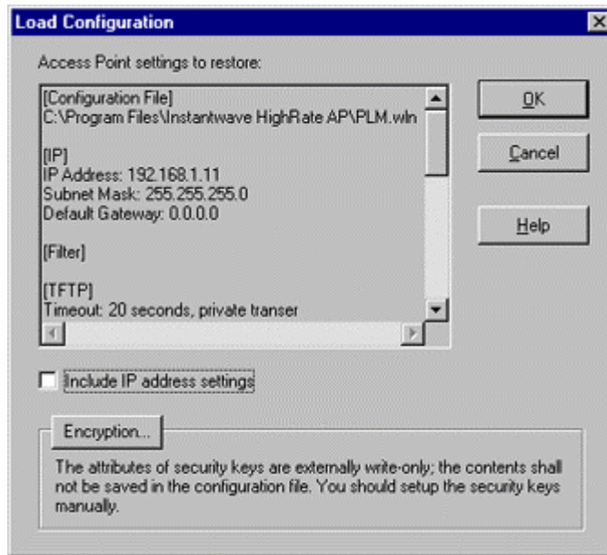
Figure 41. Load Configuration
