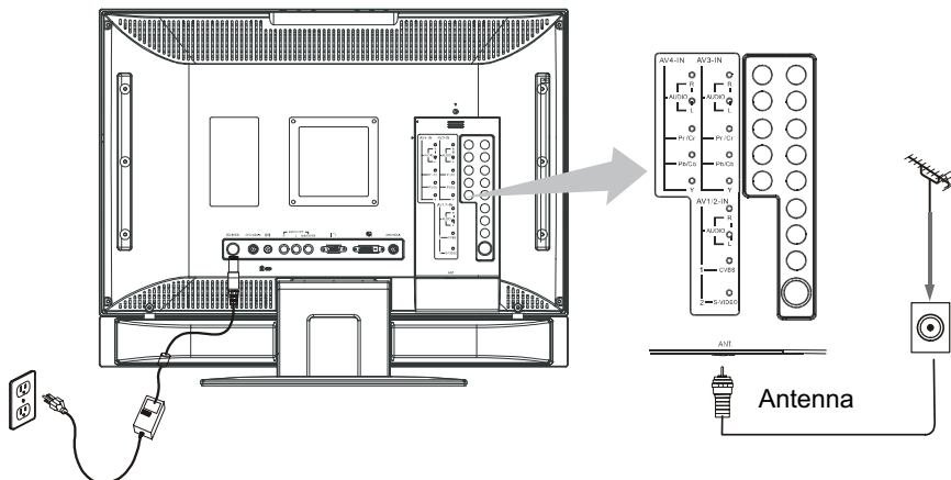
Monitor rear panel
