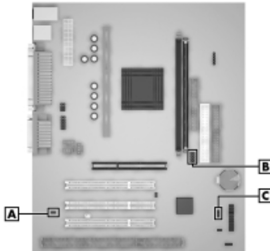
Locating system board jumpers
