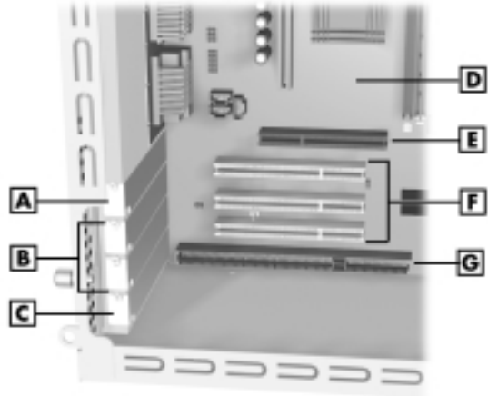
Locating expansion board slots and connectors
